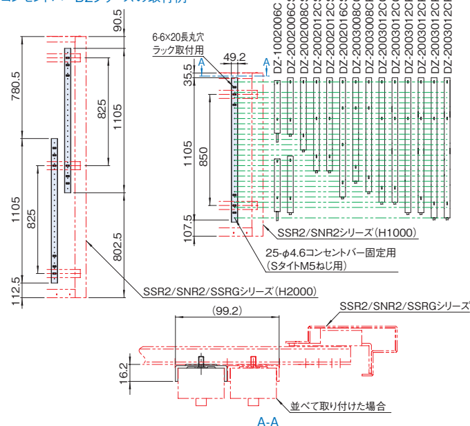
DZO-850JB consent bar DZ series of the attachment example
