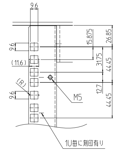
C部詳細 (1 : 3)
