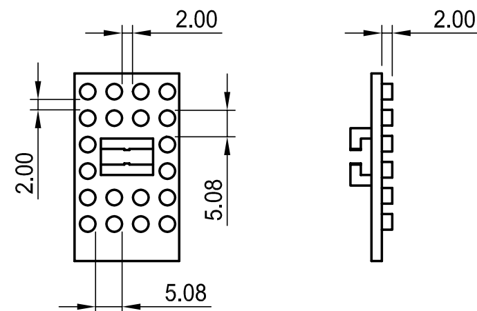
Karten-Igel A 91 99 000 Card guide A 91 99 000
