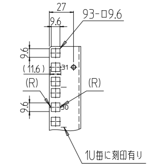
D部詳細 (1:4)
