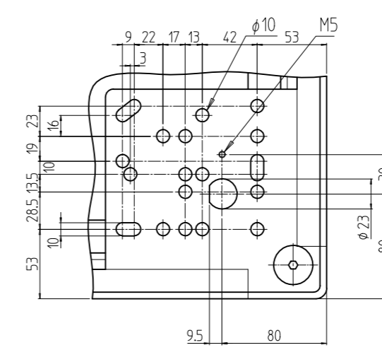
B部詳細 (1:4)
