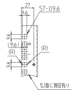
C部詳細 (1:4)
