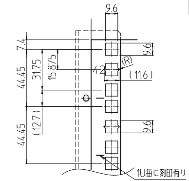
A部詳細 (1:3)
