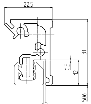
B部詳細 (1 : 1)
