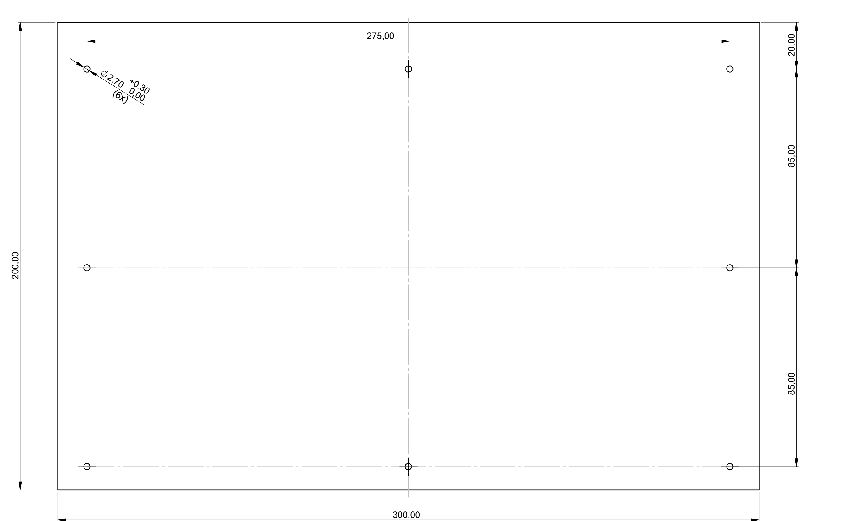
Platine Bedienfront P C B Operating panel
