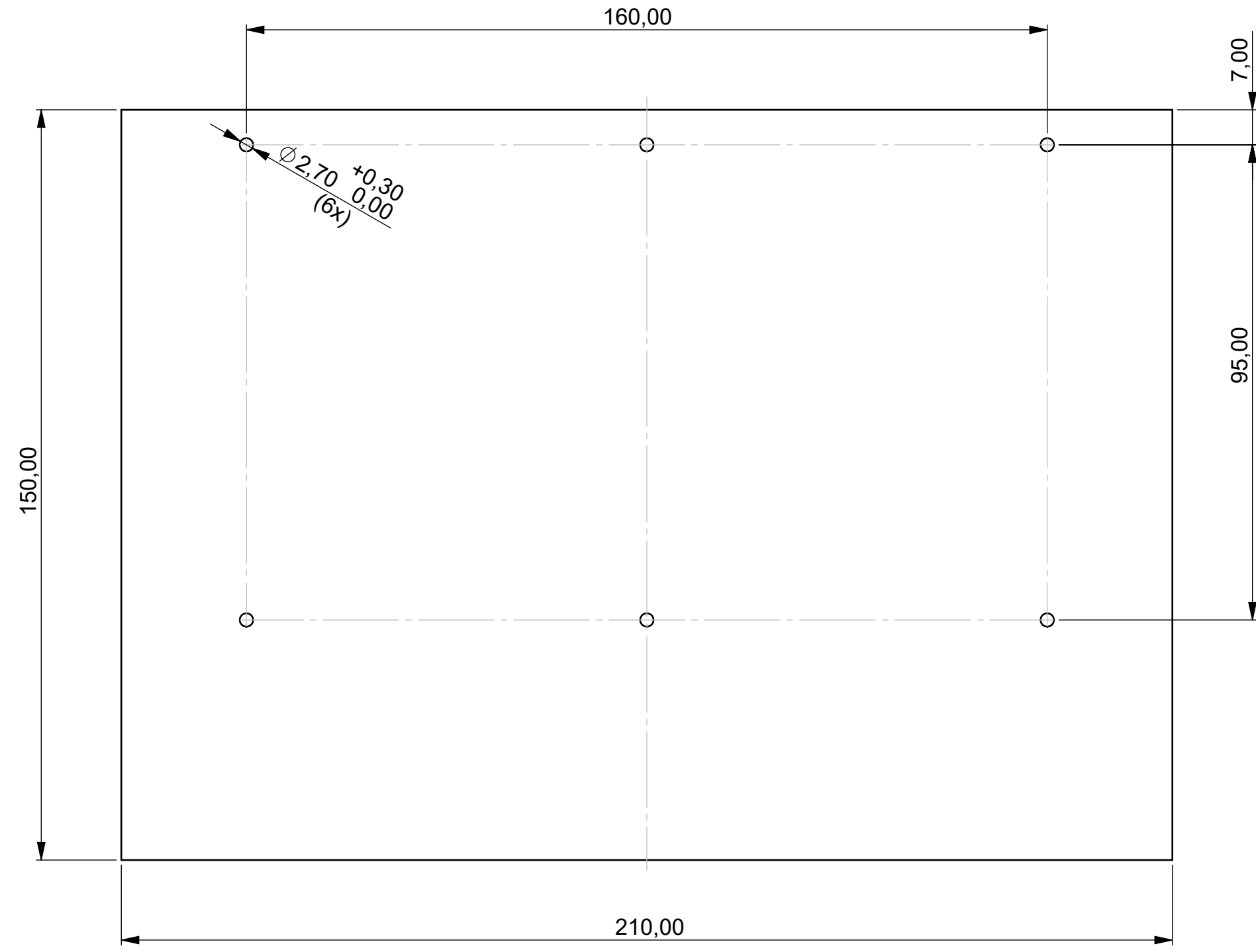
Platine Bodenplatte P C B Bottom panel
