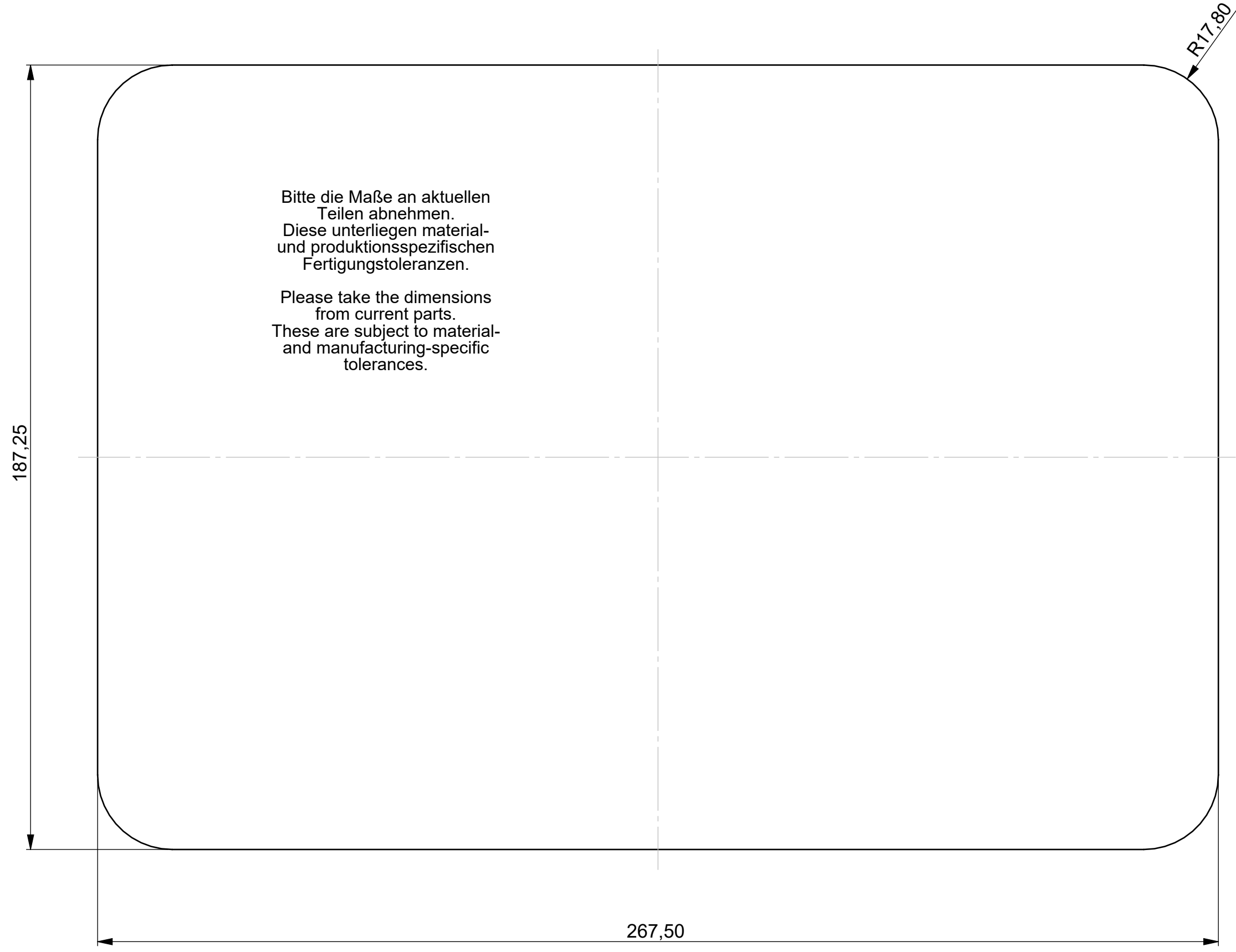
Folientastatur membrane keyboard
