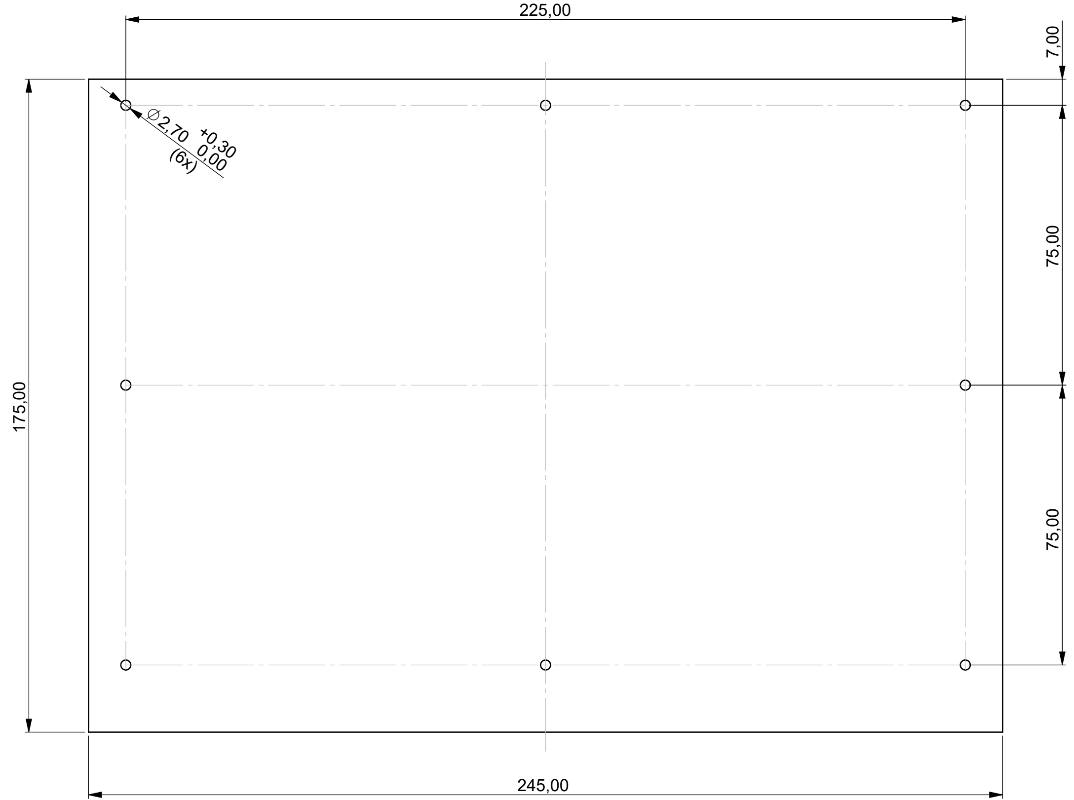
Platine Bedienfront P C B Operating panel
