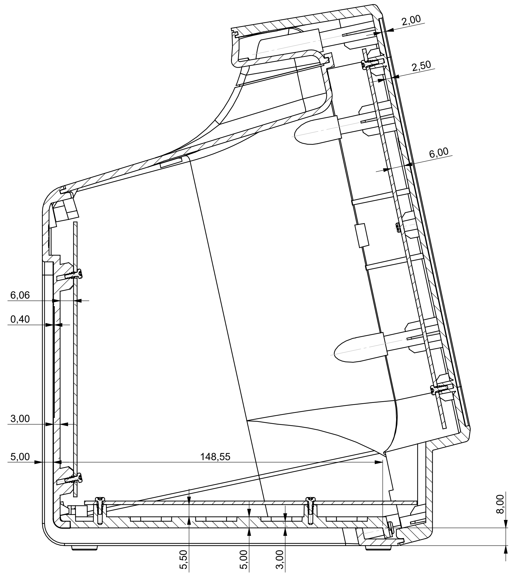
Platine Bedienfront P C B Operating panel
