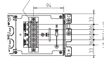
INSIDE VIEW OF TB COVER (REAR)
