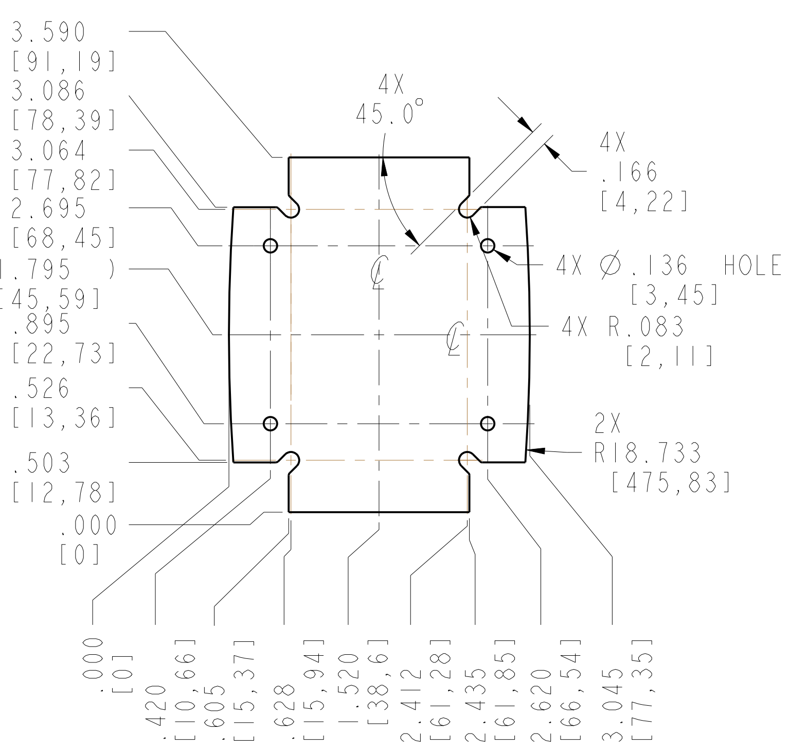
PCB BOARD (TOP COVER) MAX PCB SIZE, .063 TK
