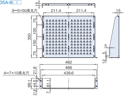
RSEH-2U35A-B□□
