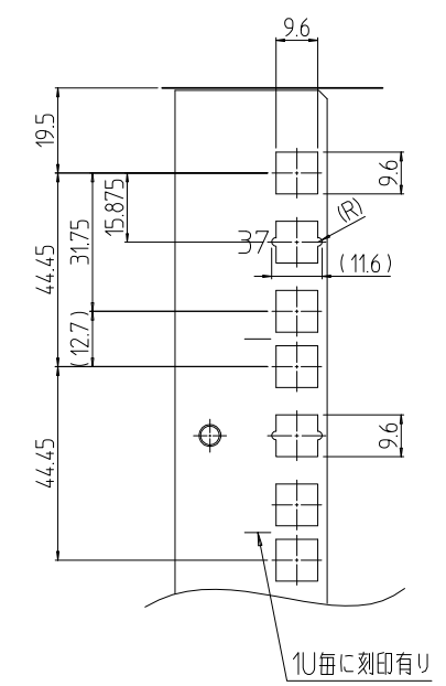
A部詳細 (1:2)
