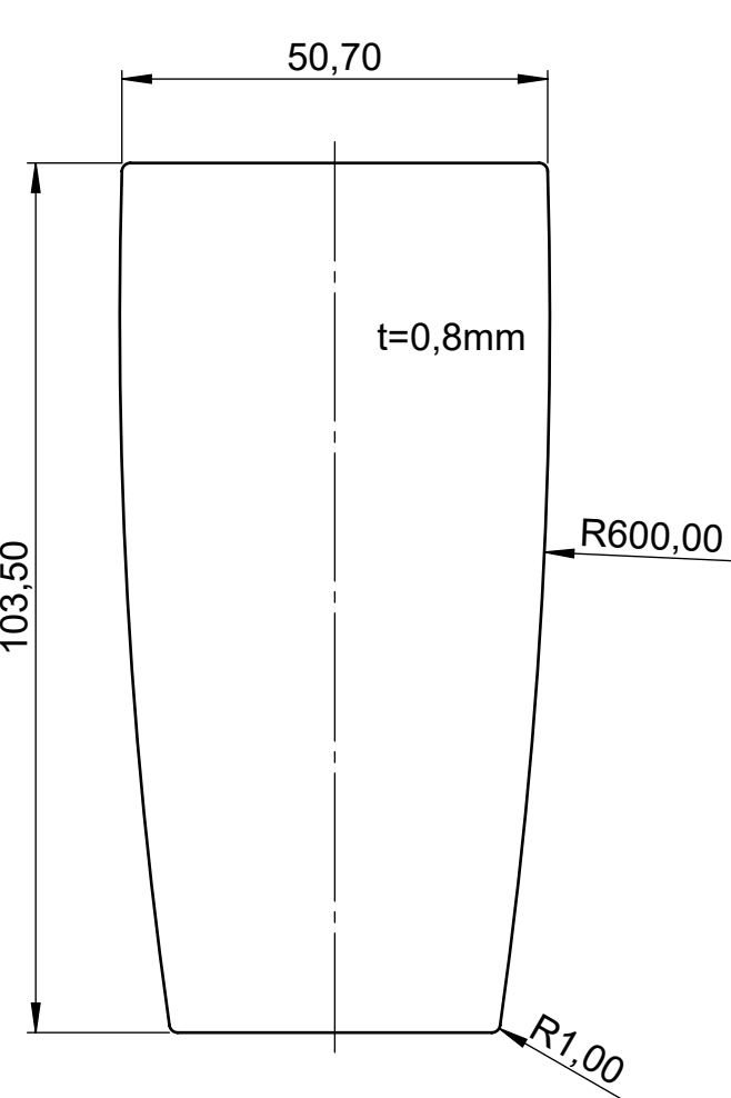
Folientastatur membrane keyboard
