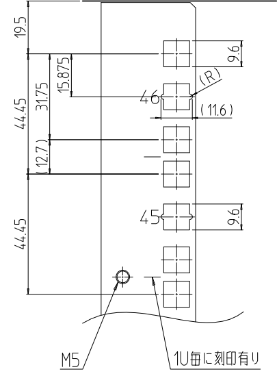
B部詳細 (1:2)
